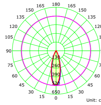
Average Diffuse Angle(50%): 29.6° Unit: cd C0-C180 C90-C270 G0 Illuminance at a Distance 4000K
