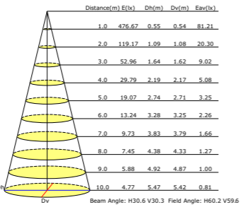
Average Diffuse Angle(50%): 30.5° Unit: cd C0-C180 C90-C270 G1 Illuminance at a Distance 3000K
