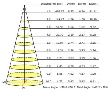
Average Diffuse Angle(50%): 30.5° Unit: cd C0-C180 C90-C270 G1 Illuminance at a Distance 2700K
