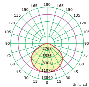
Unit: cd Average Diffuse Angle(50%): 116.1° — C0-C180 — C90-C270 — G1
