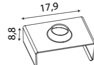
Clip aluminium
