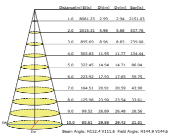
Beam Angle: H112.4 V111.6 Field Angle: H144.9 V144.6
