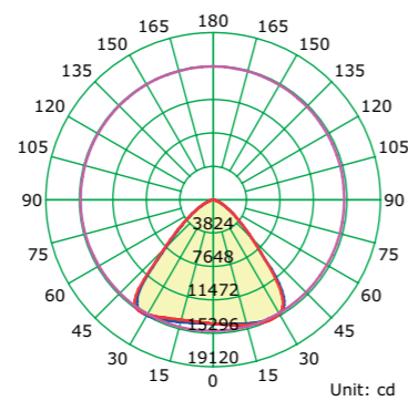
Unit: cd Average Diffuse Angle(50%): 88.1° — C0-C180 — C90-C270 — G31
