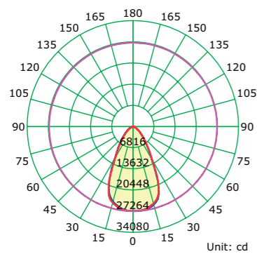
Unit: cd Average Diffuse Angle(50%): 56.8° — C0-C180 — C90-C270 — G5
