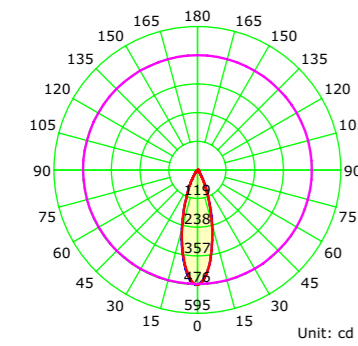
Average Diffuse Angle(50%): 30.5° Unit: cd C0-C180 C90-C270 G1 Illuminance at a Distance 2700K
