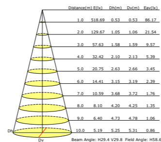
Average Diffuse Angle(50%): 29.6° Unit: cd C0-C180 C90-C270 G0 Illuminance at a Distance 4000K
