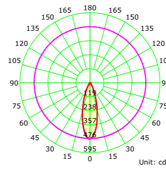
Average Diffuse Angle(50%): 30.5° Unit: cd C0-C180 C90-C270 G1 Illuminance at a Distance 3000K
